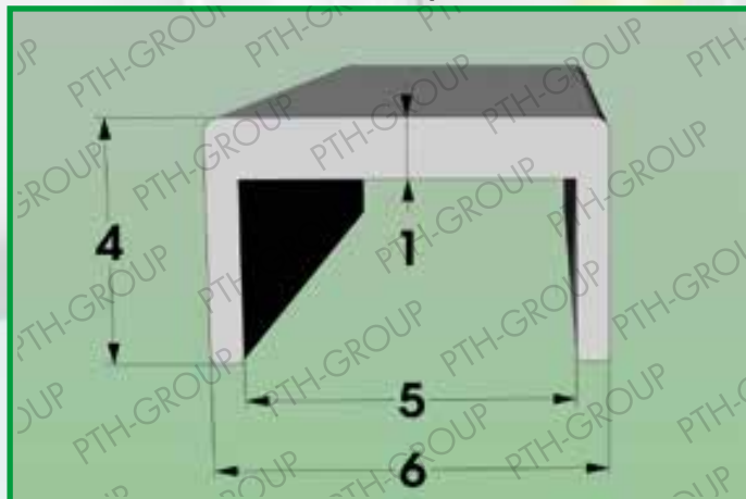
Profile 1010.509 Material: POLYCARBONATE CLEAR / OPAL PMMA CLEAR / OPAL
