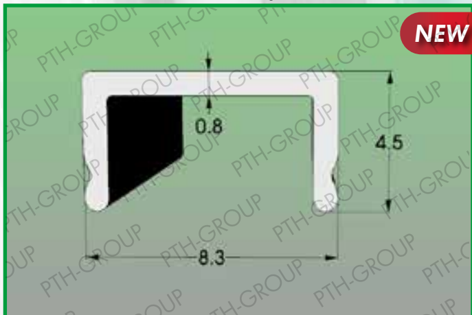
Profile 1010.583 Material: POLYCARBONATE CLEAR / OPAL / SATIN SBB PMMA CLEAR / SATIN
