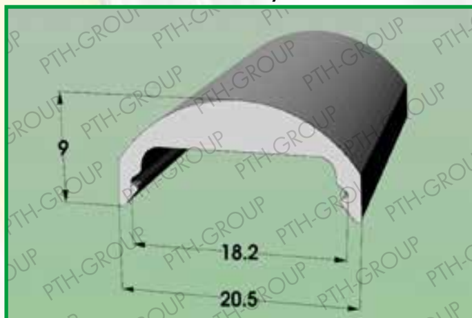
Profile 1010.119 Material: POLYCARBONATE CLEAR PMMA CLEAR / SATIN
