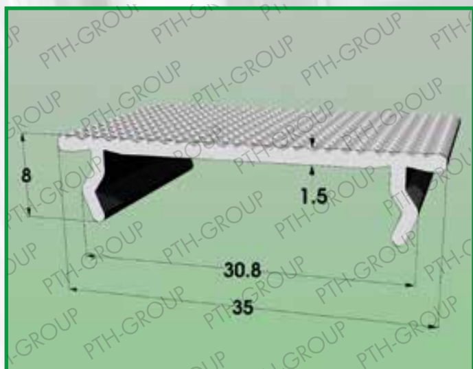
Profile 1010.319 Material: POLYCARBONATE
