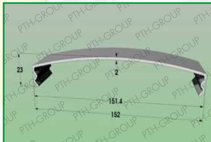
Profile 1010.78 Material: POLYCARBONATE CLEAR / OPAL
