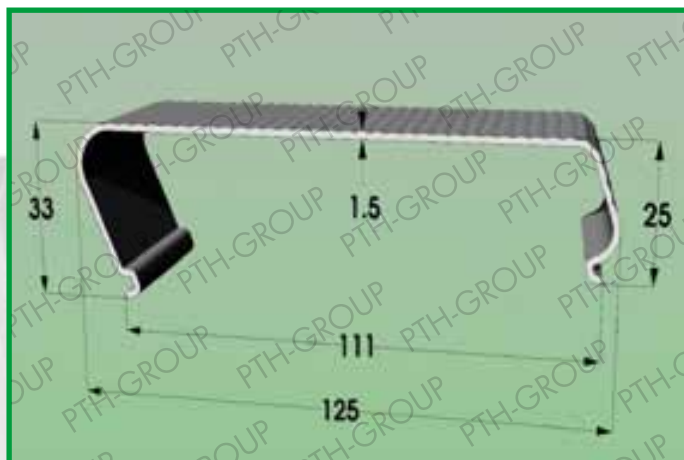
Profile 1010.36 Material: POLYCARBONATE CLEAR / OPAL
