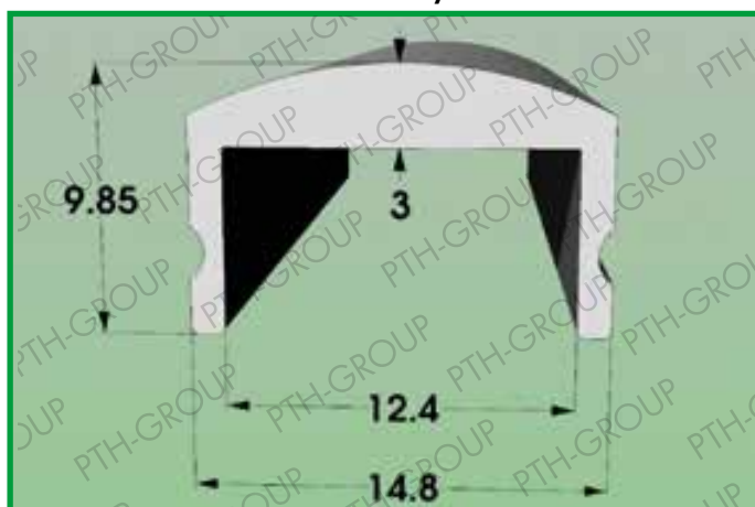
Profile 1010.410 Material: POLYCARBONATE CLEAR / OPAL PMMA CLEAR / SATIN
