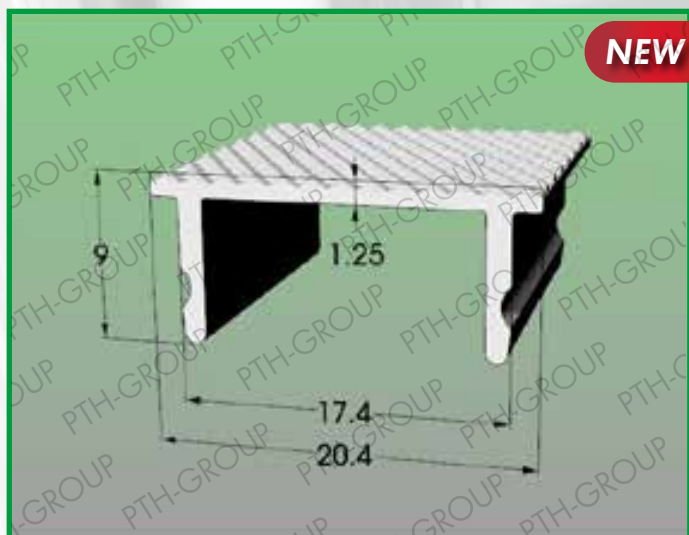
Profile 1010.570 Material: POLYCARBONATE
