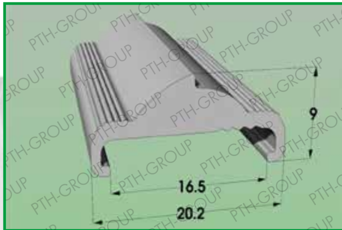
Profile 1010.313 Material: PMMA CLEAR / SATIN
