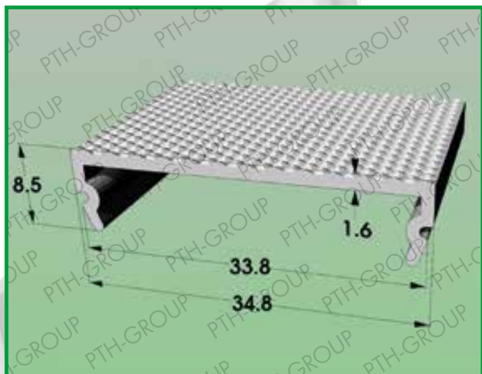
Profile 1010.180 Material: POLYCARBONATE
