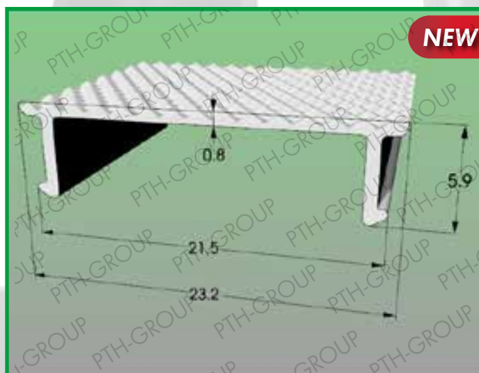
Profile 1010.580 Material: POLYCARBONATE
