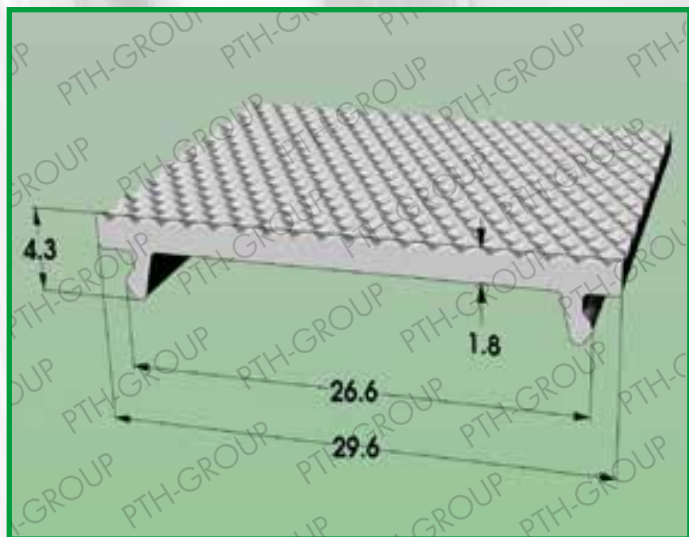
Profile 1010.260 Material: POLYCARBONATE
