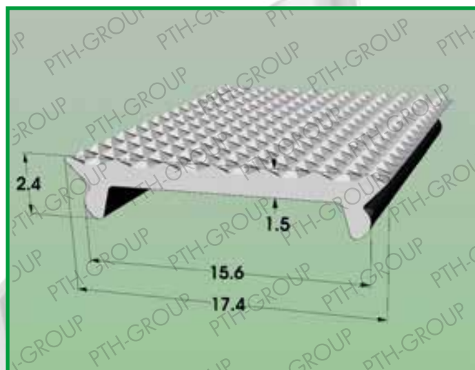
Profile 1010.420 Material: POLYCARBONATE
