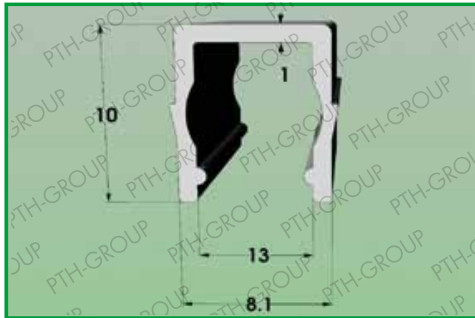
Profile 1010.288 Material: POLYCARBONATE
