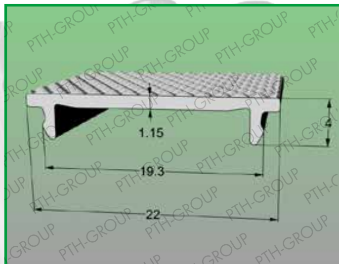
Profile 1010.519 Material: POLYCARBONATE
