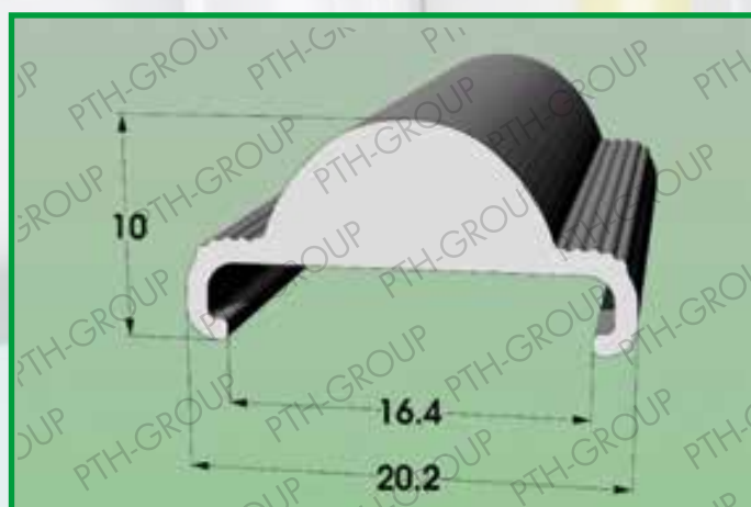
Profile 1010.270 Material: PMMA CLEAR / SATIN
