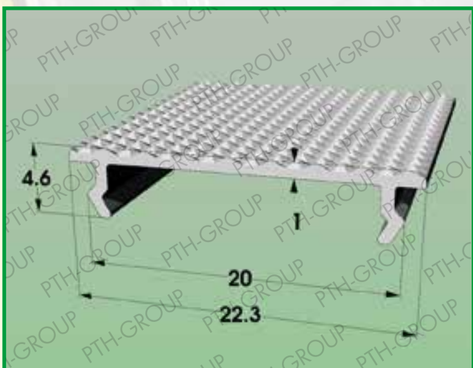
Profile 1010.394 Material: POLYCARBONATE
