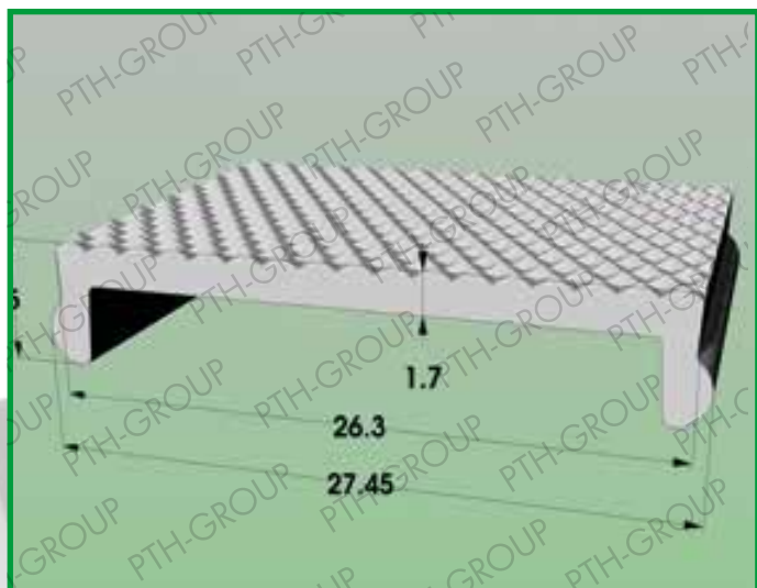
Profile 1010.512 Material: POLYCARBONATE
