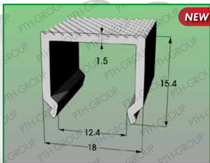
Profile 1010.561 Material: POLYCARBONATE
