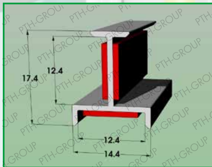
Profile 1010.466 Material: POLYCARBONATE
