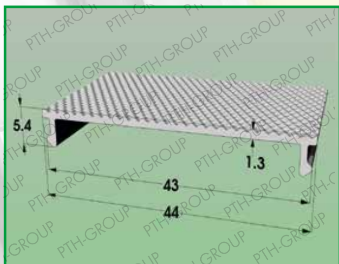
Profile 1010.268 Material: POLYCARBONATE
