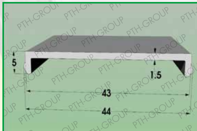
Profile 1010.269 Material: PMMA CLEAR / SATIN
