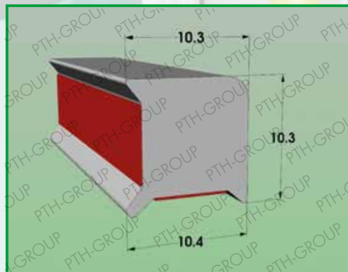
Profile 1010.19 Material: POLYCARBONATE
