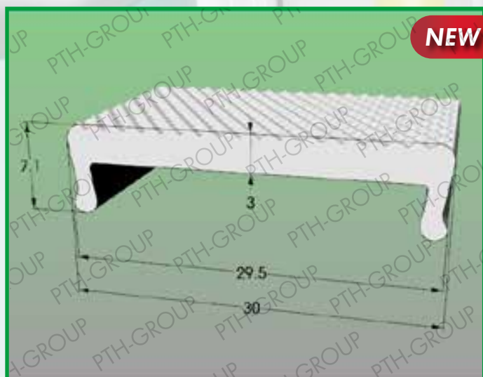
Profile 1010.574 Material: POLYCARBONATE
