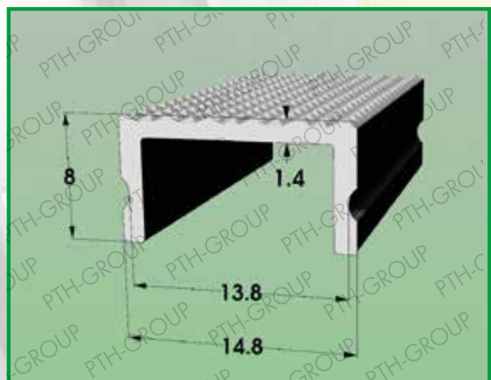
Profile 1010.146 Material: POLYCARBONATE
