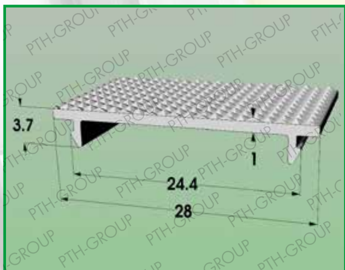
Profile 1010.162 Material: POLYCARBONATE
