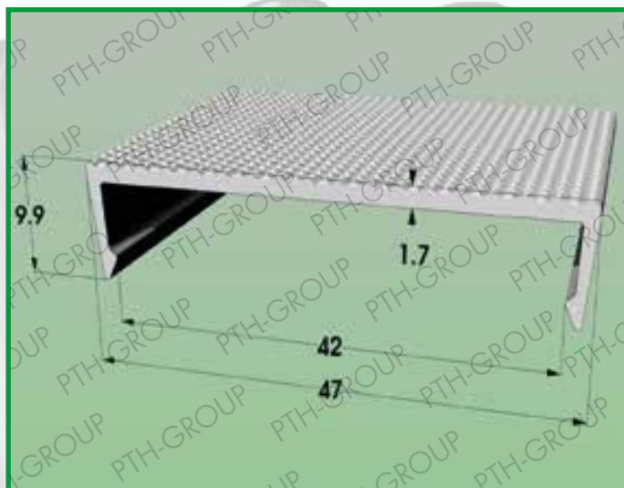
Profile 1010.412 Material: POLYCARBONATE
