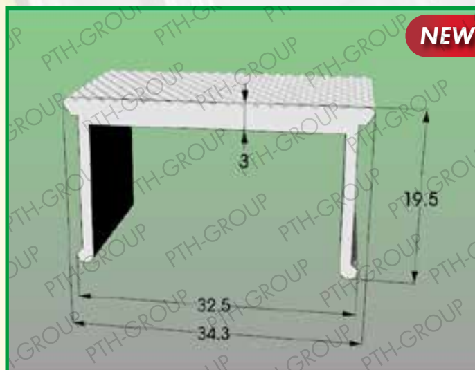
Profile 1010.581 Material: POLYCARBONATE
