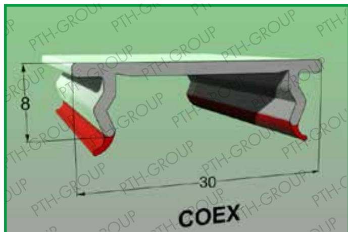
Profile 1010.318 model B Material: POLYCARBONATE + SOFT LAYER
