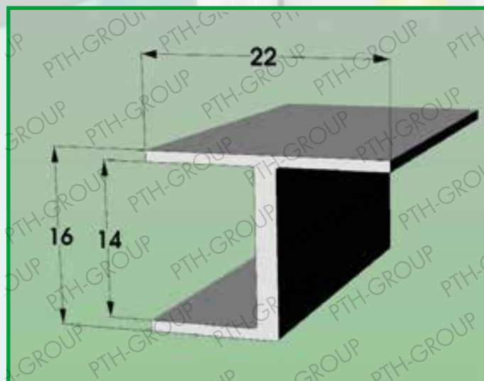
Profile 1010.105 Material: POLYCARBONATE
