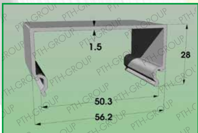
Profile 1010.375 Material: PMMA CLEAR / SATIN
